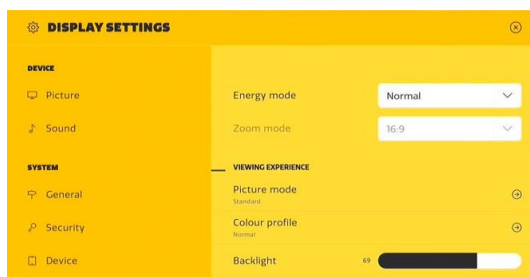
Display settings
