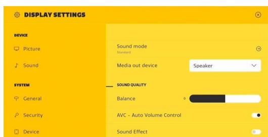
Sound settings
