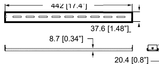
R1288-CBK Clamp Bar
