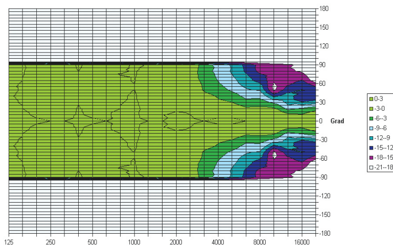
DE 100 half space Directivity Plot
