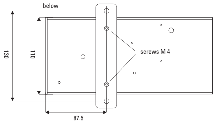
mounting bracket
