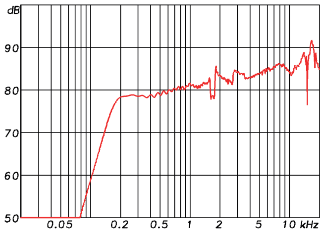
S 2 Sens. 2,83V/1m: 81,6 db (100-10k) 164 Hz - 20 kHz (-6 dB) full space
