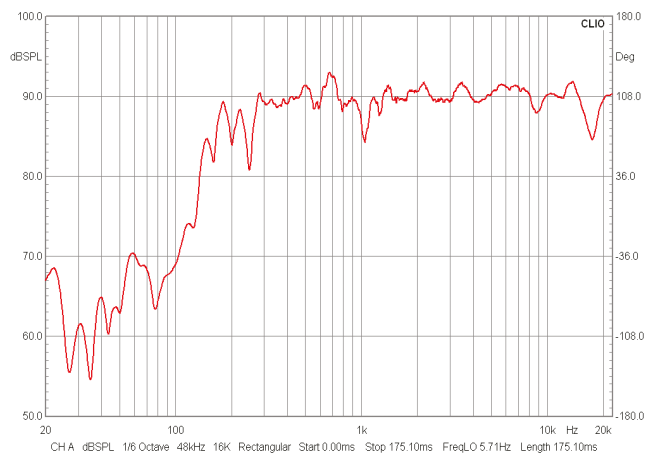
ZL 104 Sens. @ 2, 83V/1m, d=4m
