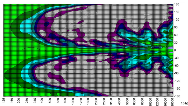
ZL 104 vert. Directivity Plot
